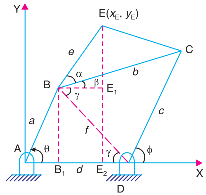
Fig. 25.3. Four bar mechanisms with a coupler point.
