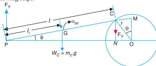
Fig. 15.23. Analytical method for inertia torque.
