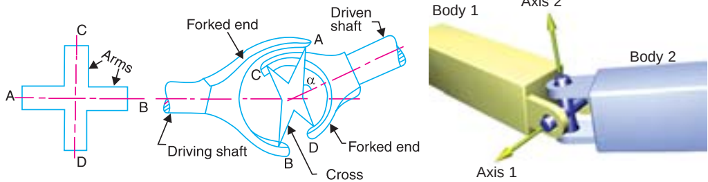
Fig. 9.18. Universal or Hooke's joint.
