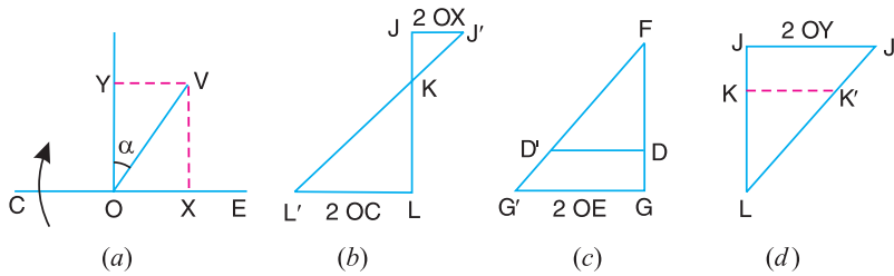
Fig. 17.40. Determination of throw and angle of advance of the virtual eccentric.
