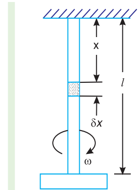
Fig 24.3. Effect of inertia of the constraint on torsional vibrations.
