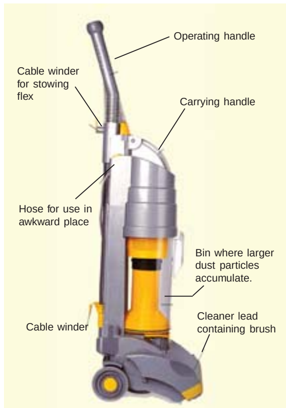
Cyclone cleaner.
