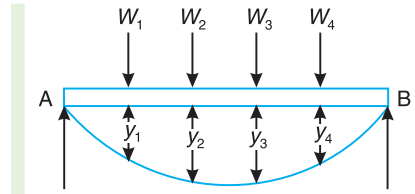
Fig. 23.11. Shaft carrying a number of point loads.
