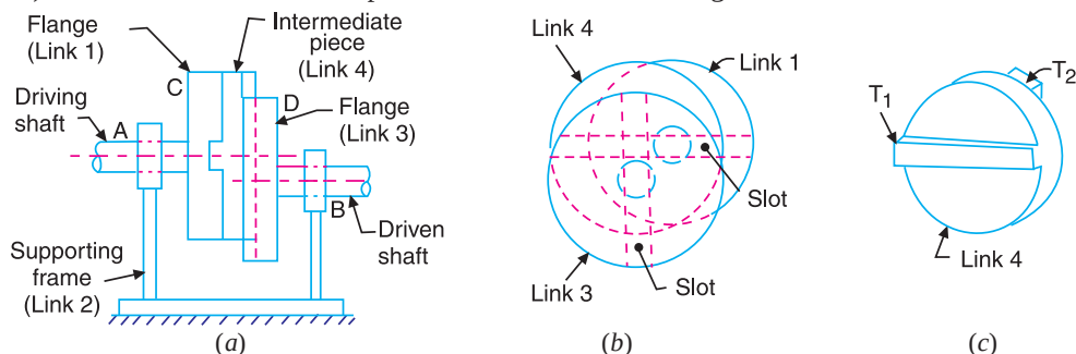
Fig. 5.36. Oldham's coupling.
