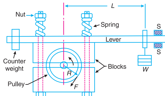
Fig. 19.31. Prony brake dynamometer.
